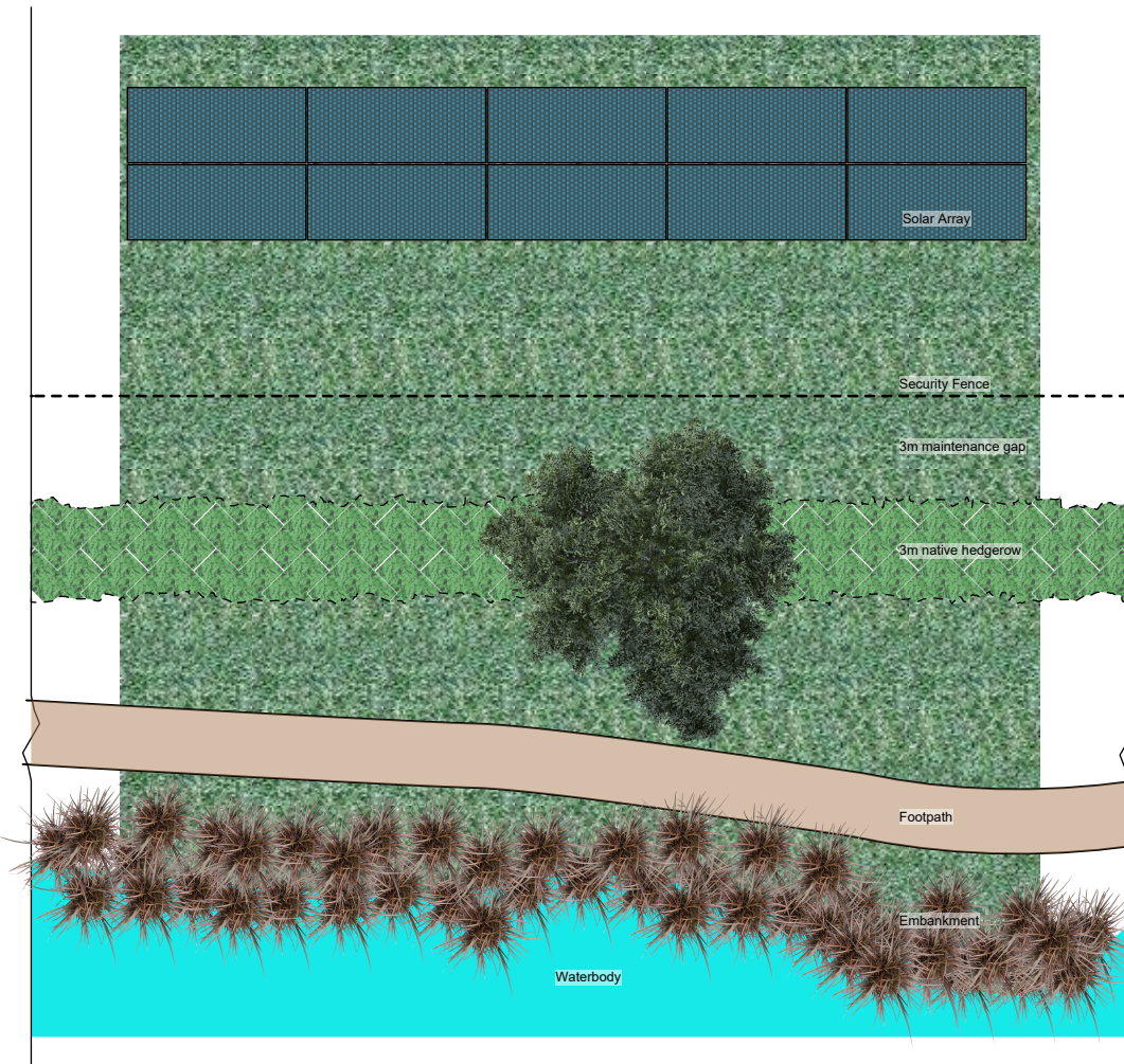
Plan View
